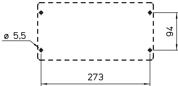
Fixing holes
